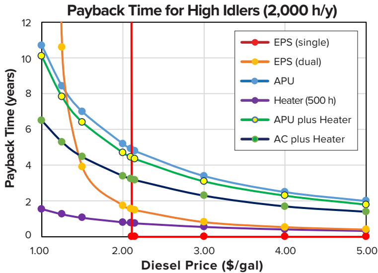
Figure 1. Equipment payback time as a function of fuel price for high idlers (2,000 h/yr). (Assumptions: idling fuel consumption = 0.8 gal/h; EPS cost, single system = $1.85/h; EPS cost, dual system = $1.00/h.)
