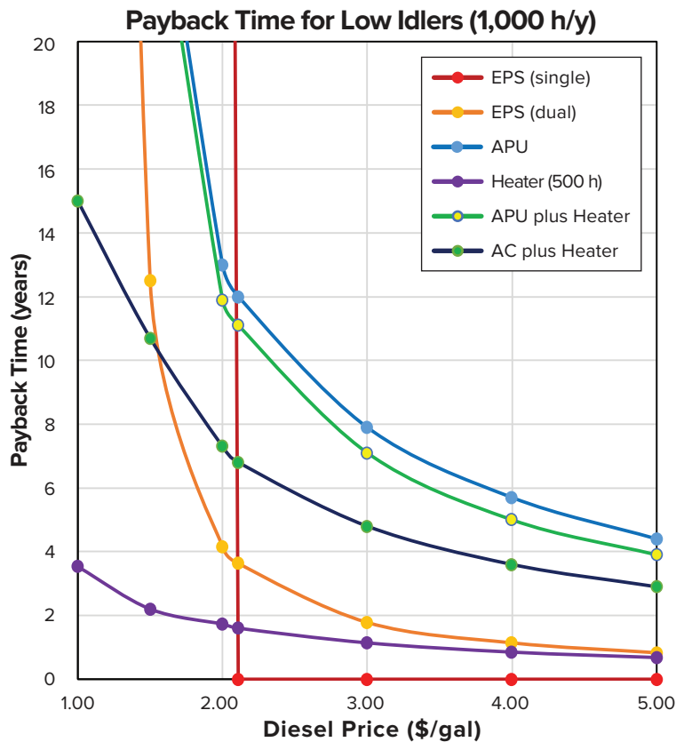
Figure 2. Equipment payback time as a function of fuel price for low idlers (1,000 h/yr). (Assumptions: idling fuel consumption = 0.8 gal/h; EPS cost, single system = $1.85/h; EPS cost, dual system = $1.00/h.)
