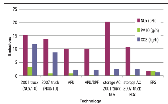
FIGURE 7. Hourly Emissions for Cooling Options, U.S. Average Location
