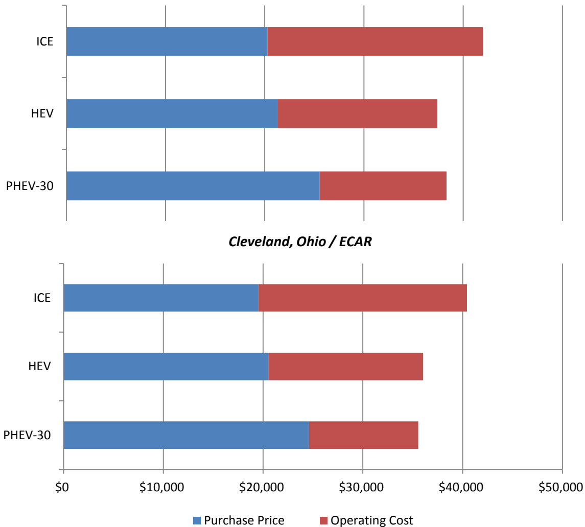
Total Lifetime Vehicle Ownership in 2030 (Net Present Value) Southern California
