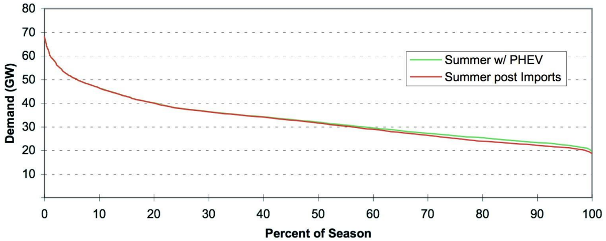
Figure 19: California summer load duration curves with and without PHEV added demand
