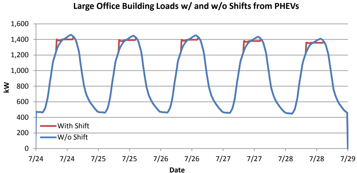
Figure J - 4: Change in load shape for July 24-29 with PHEV charging used for peak shaving.
