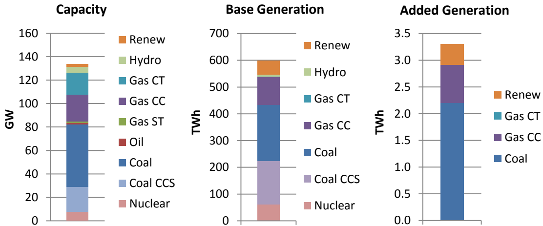
Figure 25: ECAR generating capacity, initial generation amounts, and added generation from PHEVs
