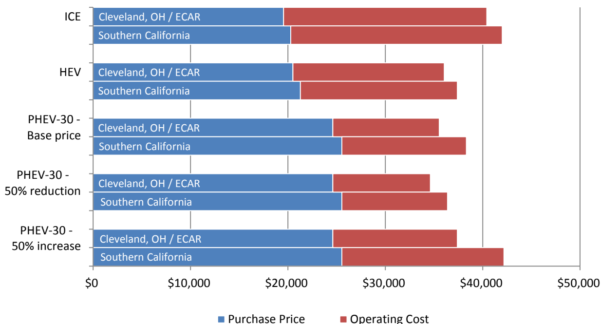
Figure 51: Effects of varying electricity costs on lifetime ownership cost
