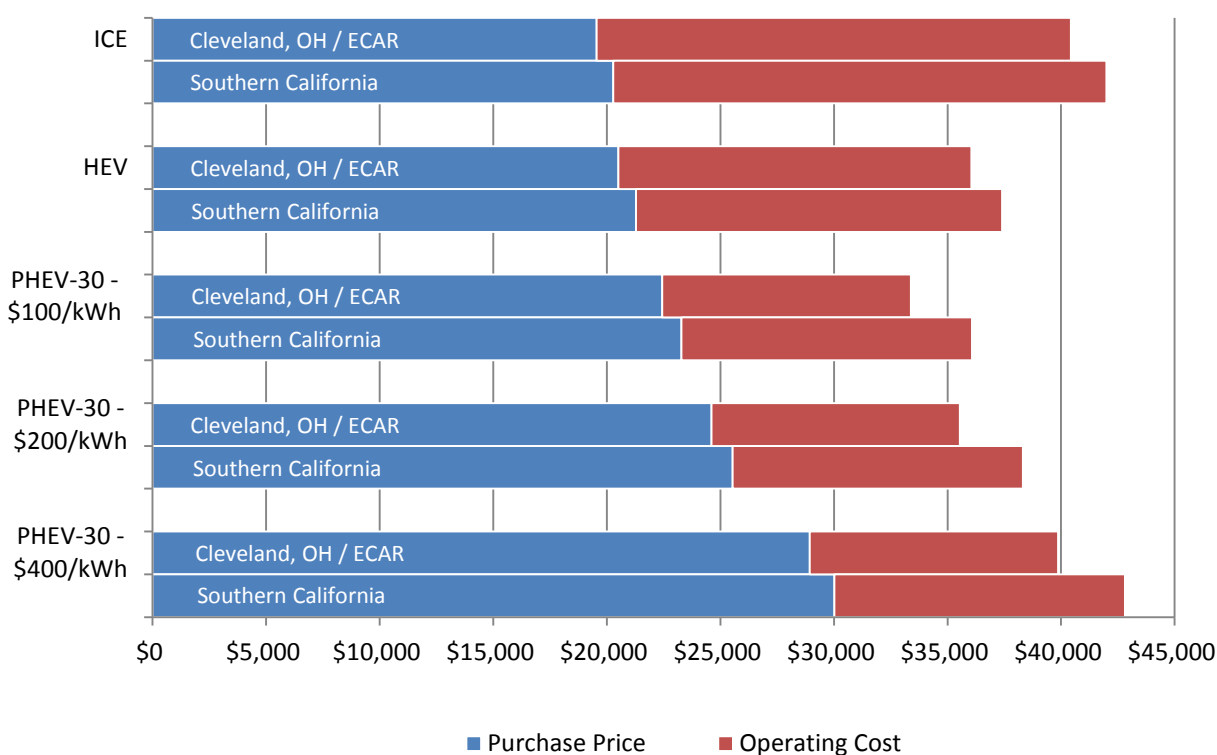
Figure 52: Effects of varying energy storage cost on lifetime ownership cost
